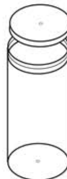
PL 128 SIZE: ø70 mmx 150 mm (H) 36 PCS PER CTN
